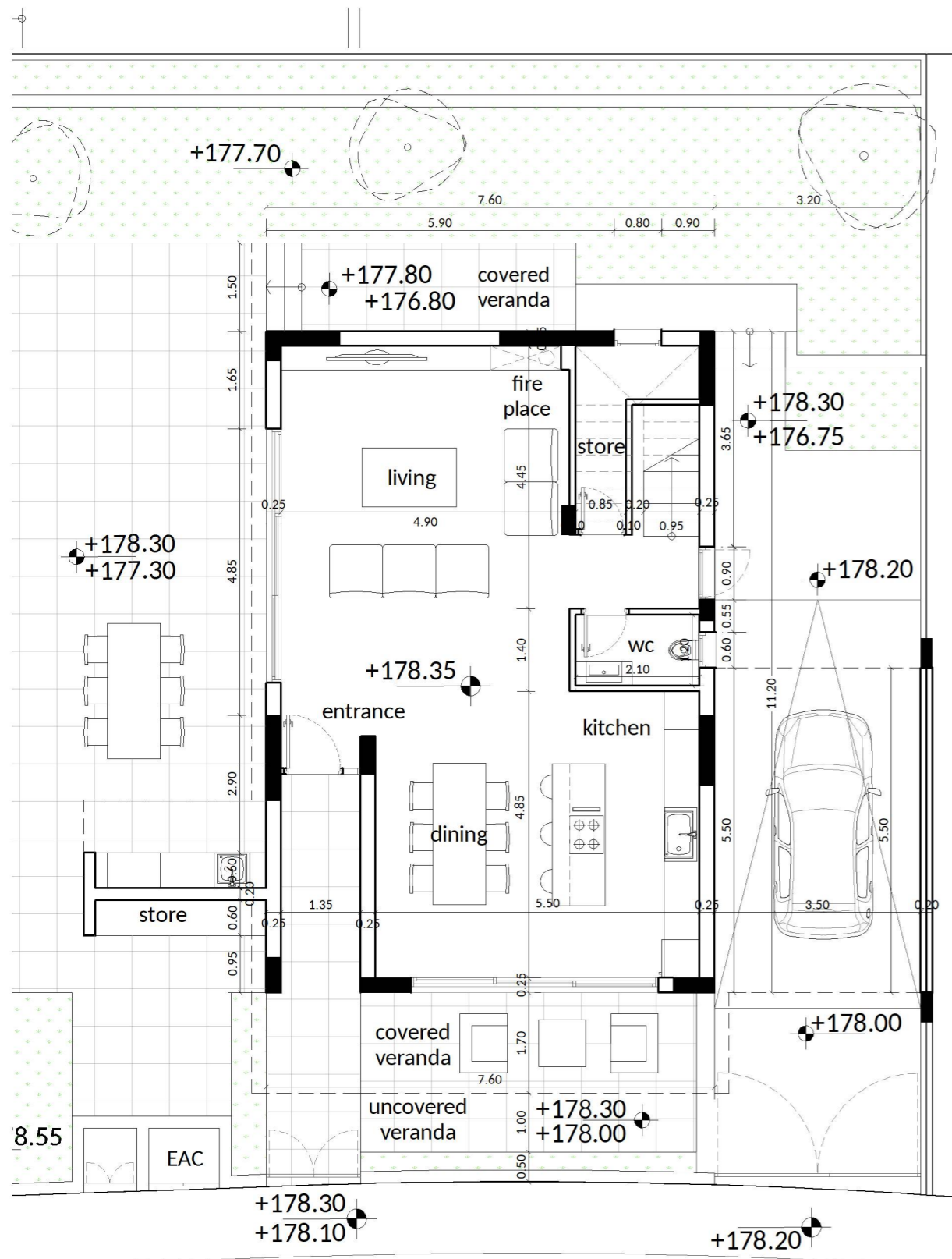
GROUND FLOOR
