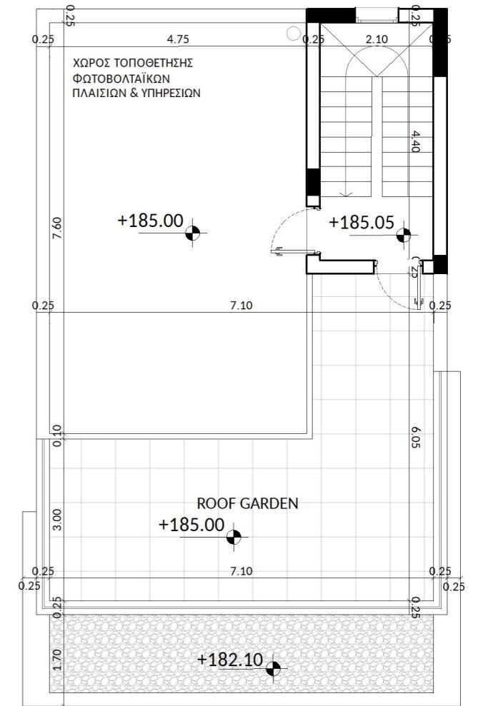
ROOF
