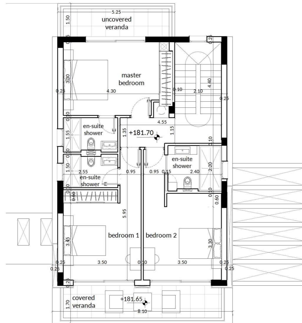
FIRST FLOOR
